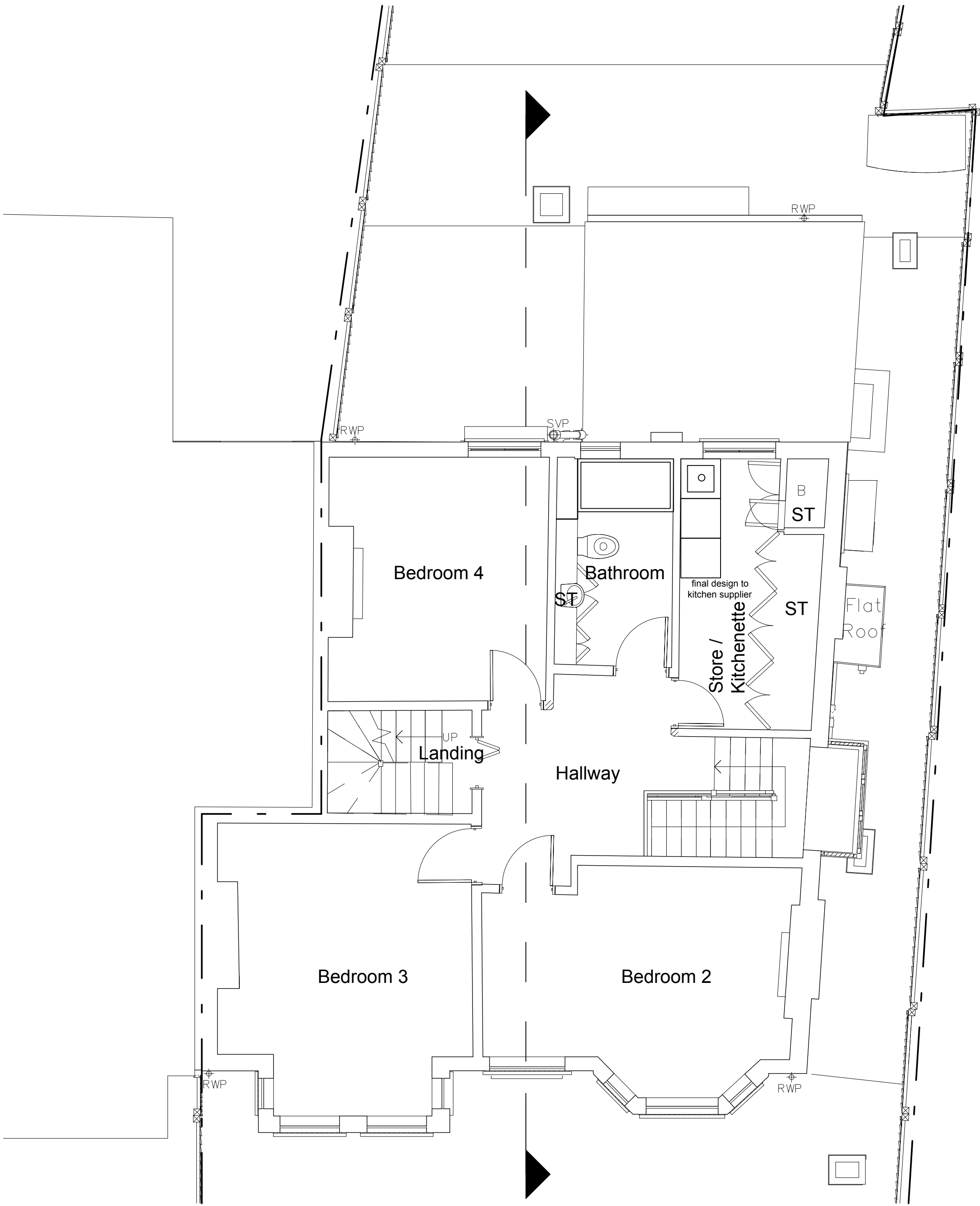
PROPOSED FIRST PLAN
