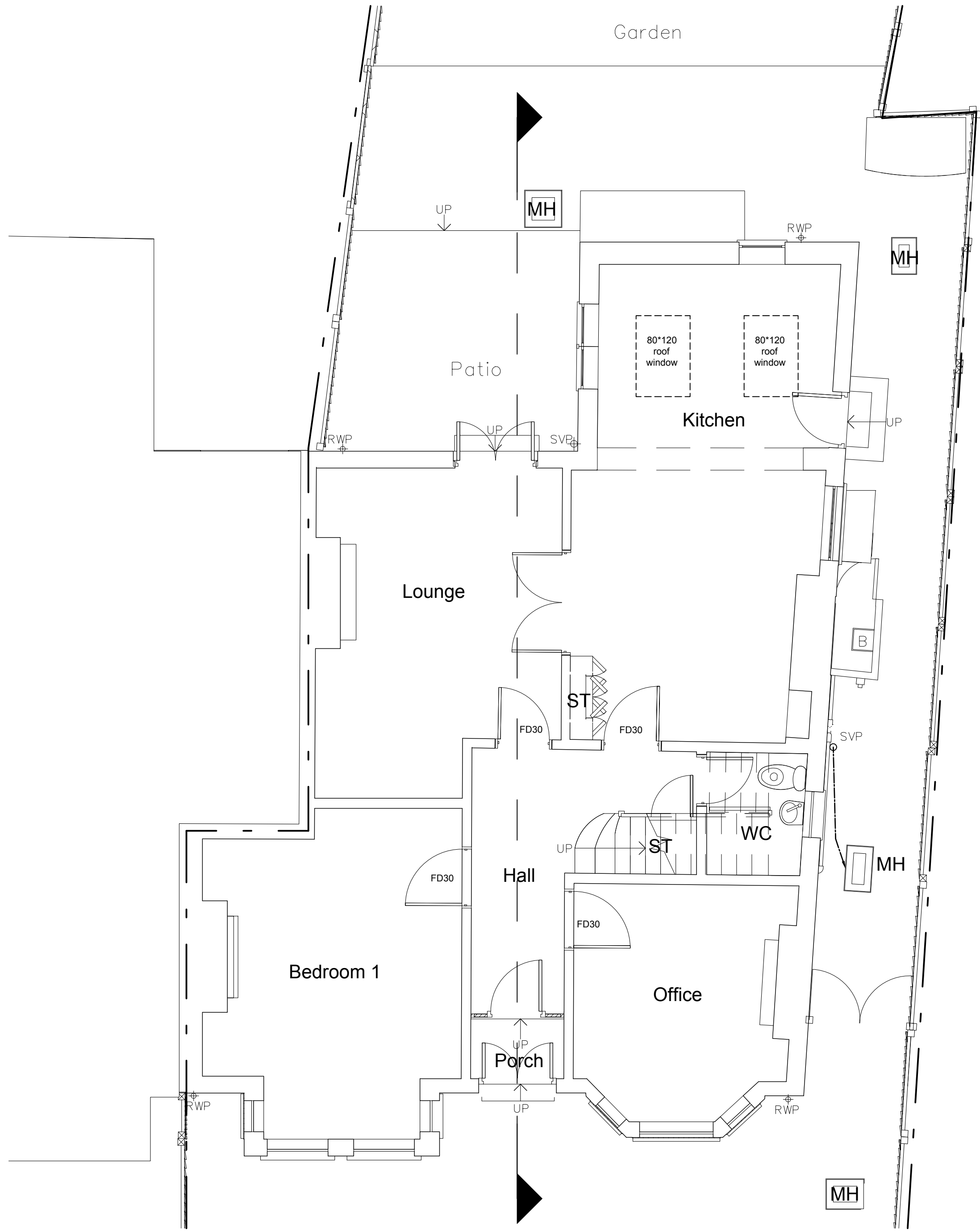
PROPOSED GROUND PLAN
